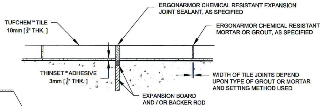
SECTION VIEW
